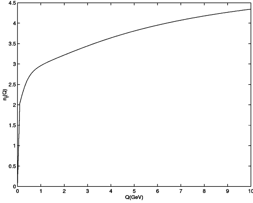
FIG. 1. The momentum dependence of n_f(Q^2) .
