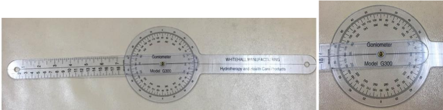
Figure 1. Standard plastic, hand-held goniometer with 1 degree markings
